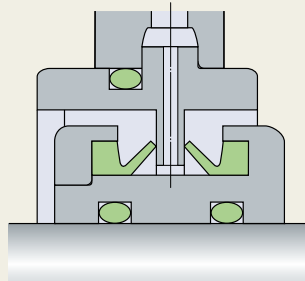
V-ring
