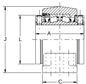
3-3/16" THRU 5" CONSTRUCTION
