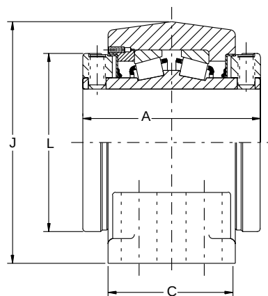
80mm THRU 125mm CONSTRUCTION
