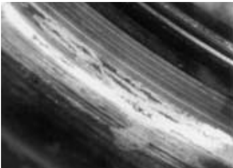
Fig. 15-13. Corrosion on Outer Ring Raceway of Deep Groove Ball Bearing
