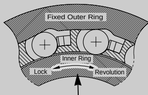
▼ Clutch Structure
