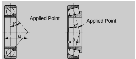
Fig. 4-6 Load Applied Point
