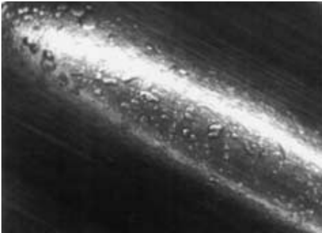
Fig. 15-11 Electric Corrosion on Outer Ring Surface of Deep Groove Ball Bearing
