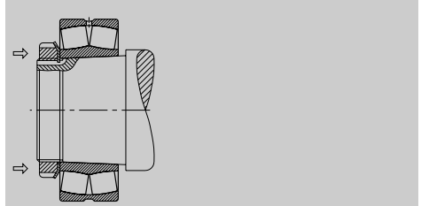
Fig. 14-4 Direct Mounting on a Tapered Shaft
