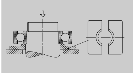
Fig. 14-9 Dismounting of Inner Ring by using Hydraulic Press
