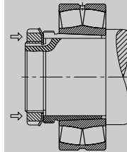
Fig. 14-6 Mounting on a Withdrawal Sleeve
