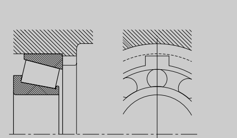
Fig. 14-16 Dismounting of Outer Ring by using Dismounting Bolt
