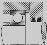
Fig. 11-7 Felt Ring
