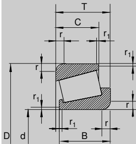
Fig. 6-2 Tapered Roller Bearings
