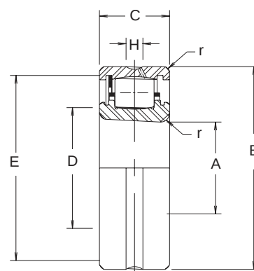
TAPERED BORE
