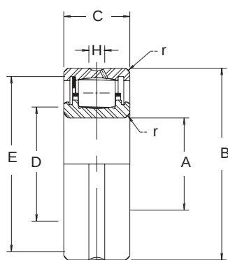
STRAIGHT BORE
